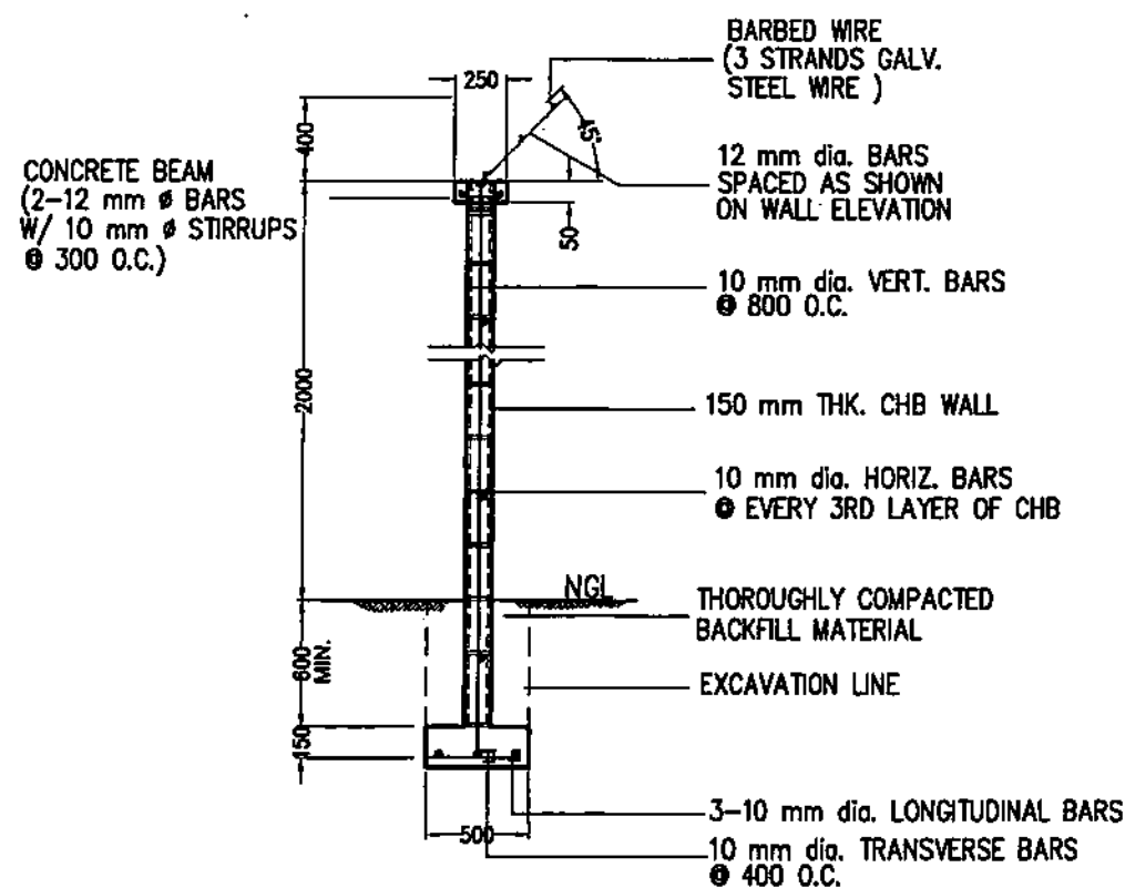
CHB WALL SECTION ON FLAT GROUND RPFB-BDC-19.002 SCALE 1:40
