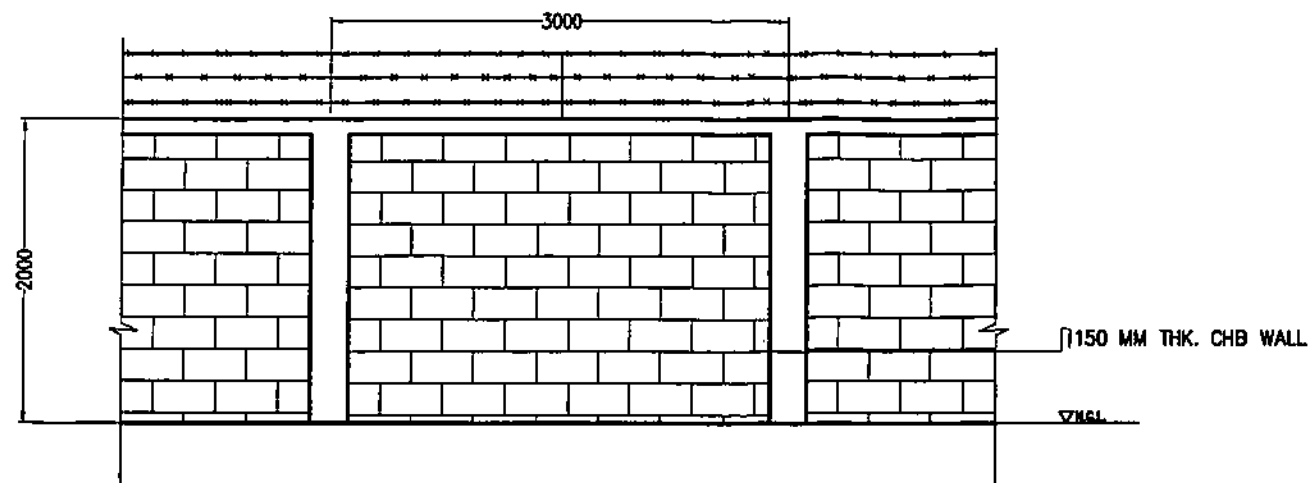
ELEVATION OF CHB FENCE RPFB-BDC-19.002 SCALE 1:50
