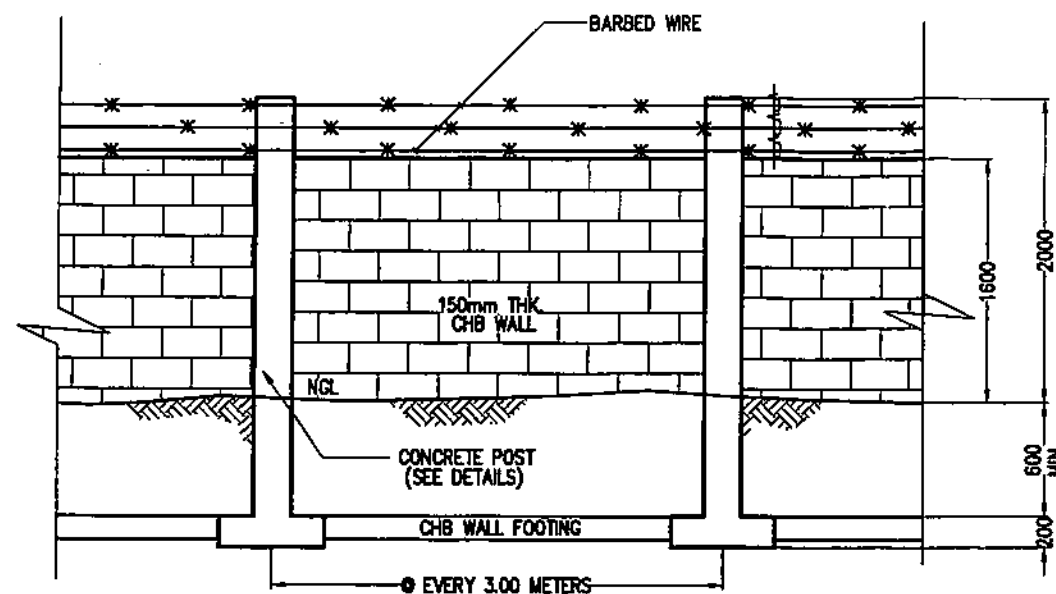
EXISTING CHB PERIMETER FENCE 1 TO BE MODIFIED
