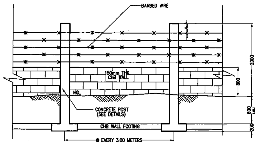
EXISTING CHB PERIMETER FENCE 2 TO BE MODIFIED
